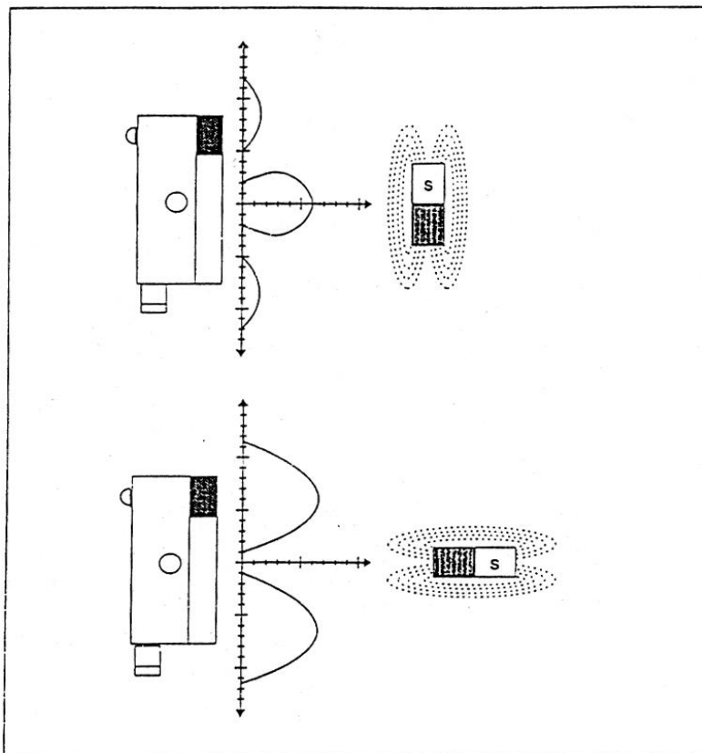
Fig. 3.3: Response characteristics of a reed proximity sensor
