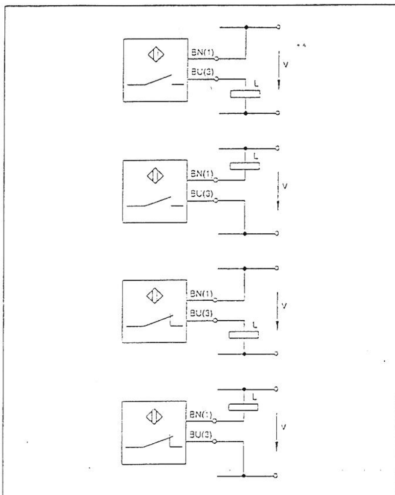
Fig. 10.1: Connection diagrams for two-wire technology (DC, AC and DC/AC [universal current] designs) V = Operating voltage, L = Load
