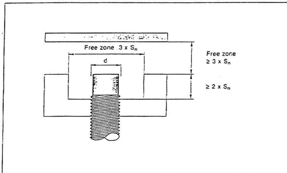
Fig. 4.6: Non-flush fitting inductive proximity sensors
