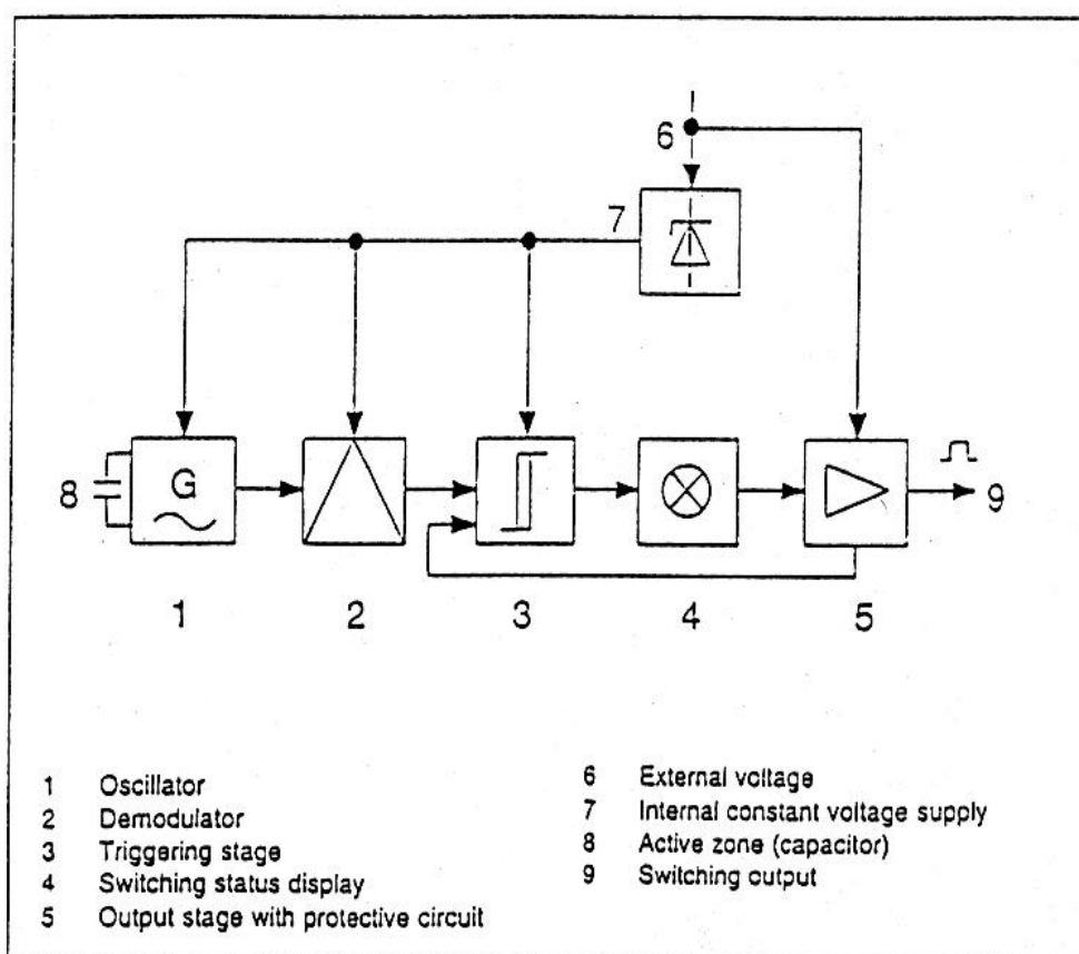
Fig. 5.1: Block circuit diagram of a capacitive proximity sensor
