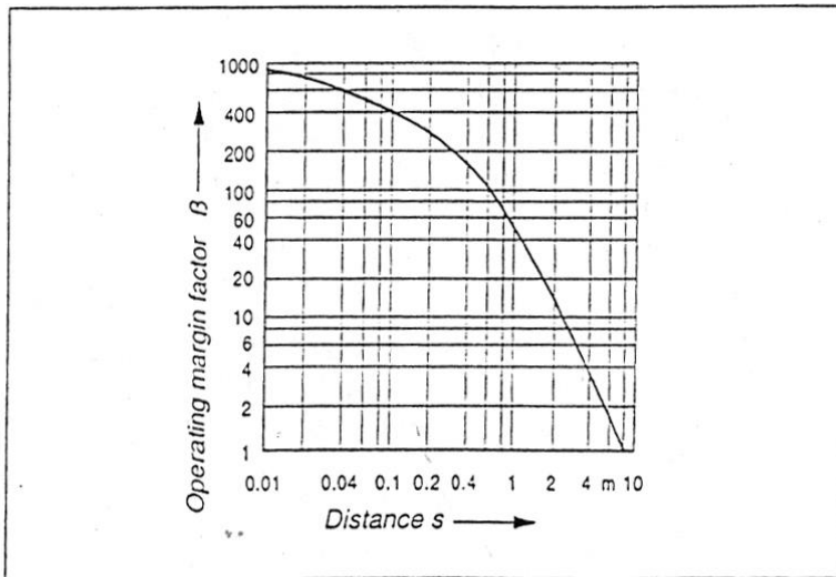
Fig. 6.3: Example showing the pattern of the operating reserve factor using a through-beam sensor
